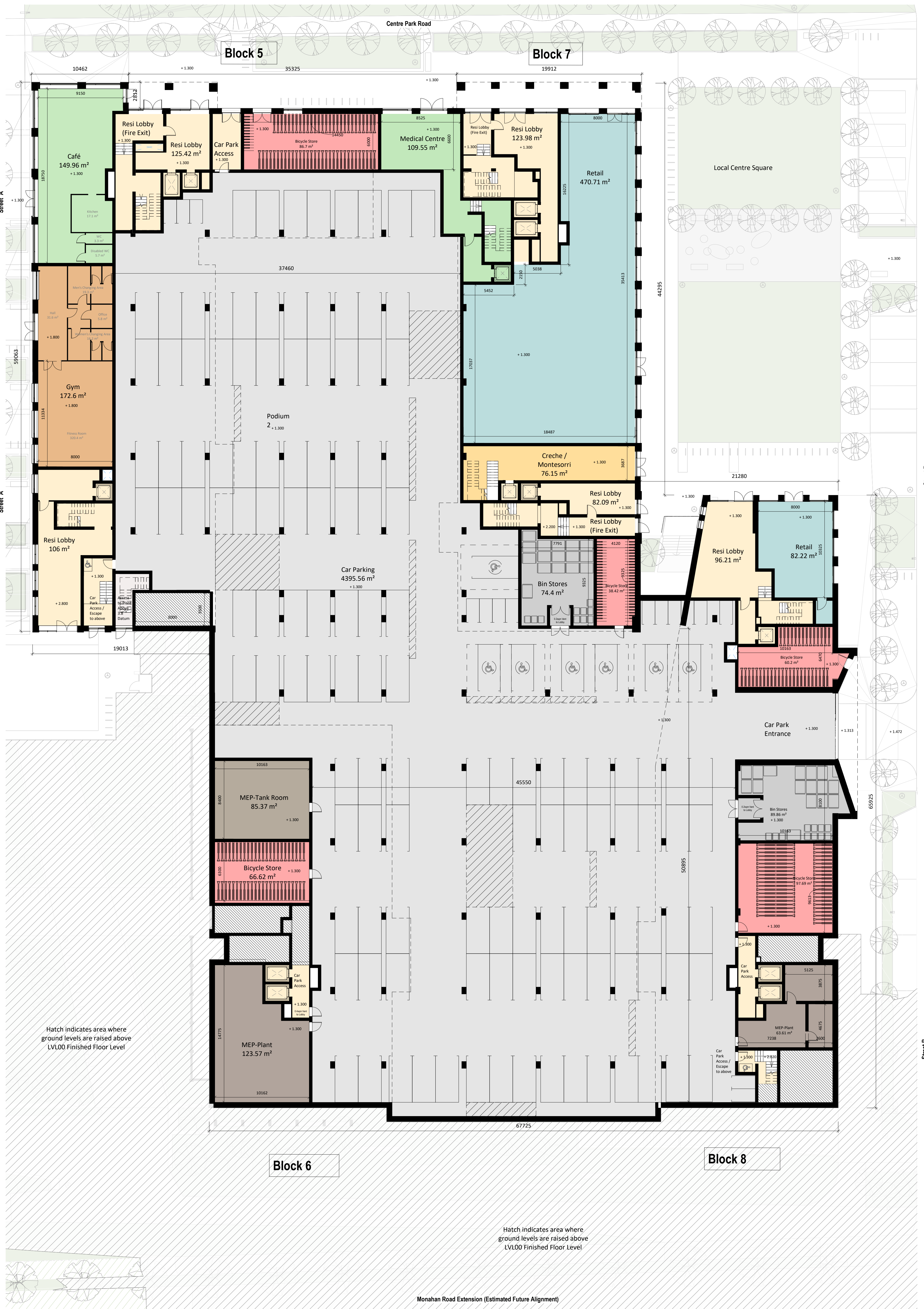
Podium 2 Level 00 Floor Plan
