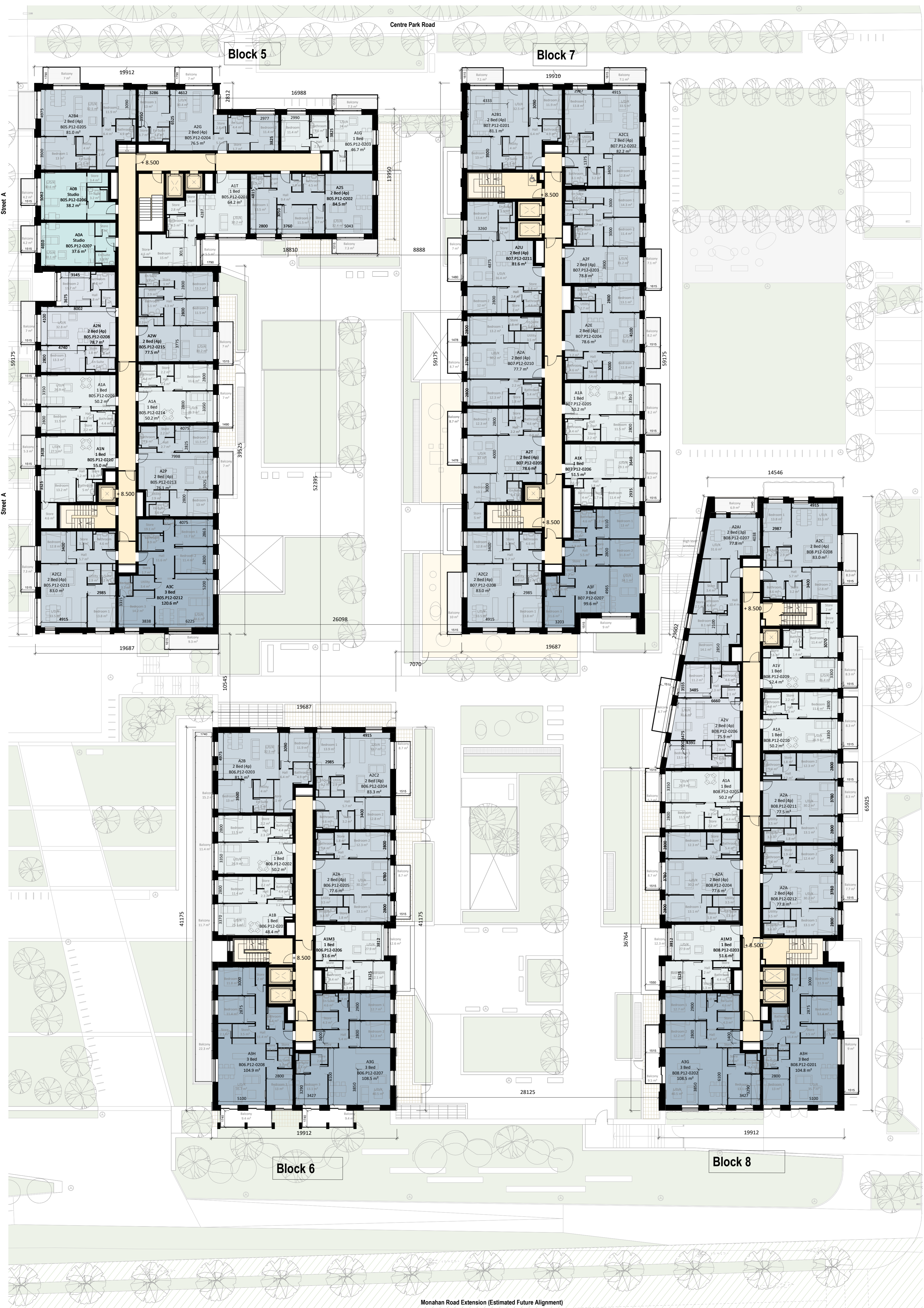
Podium 2 Level 02 Floor Plan
