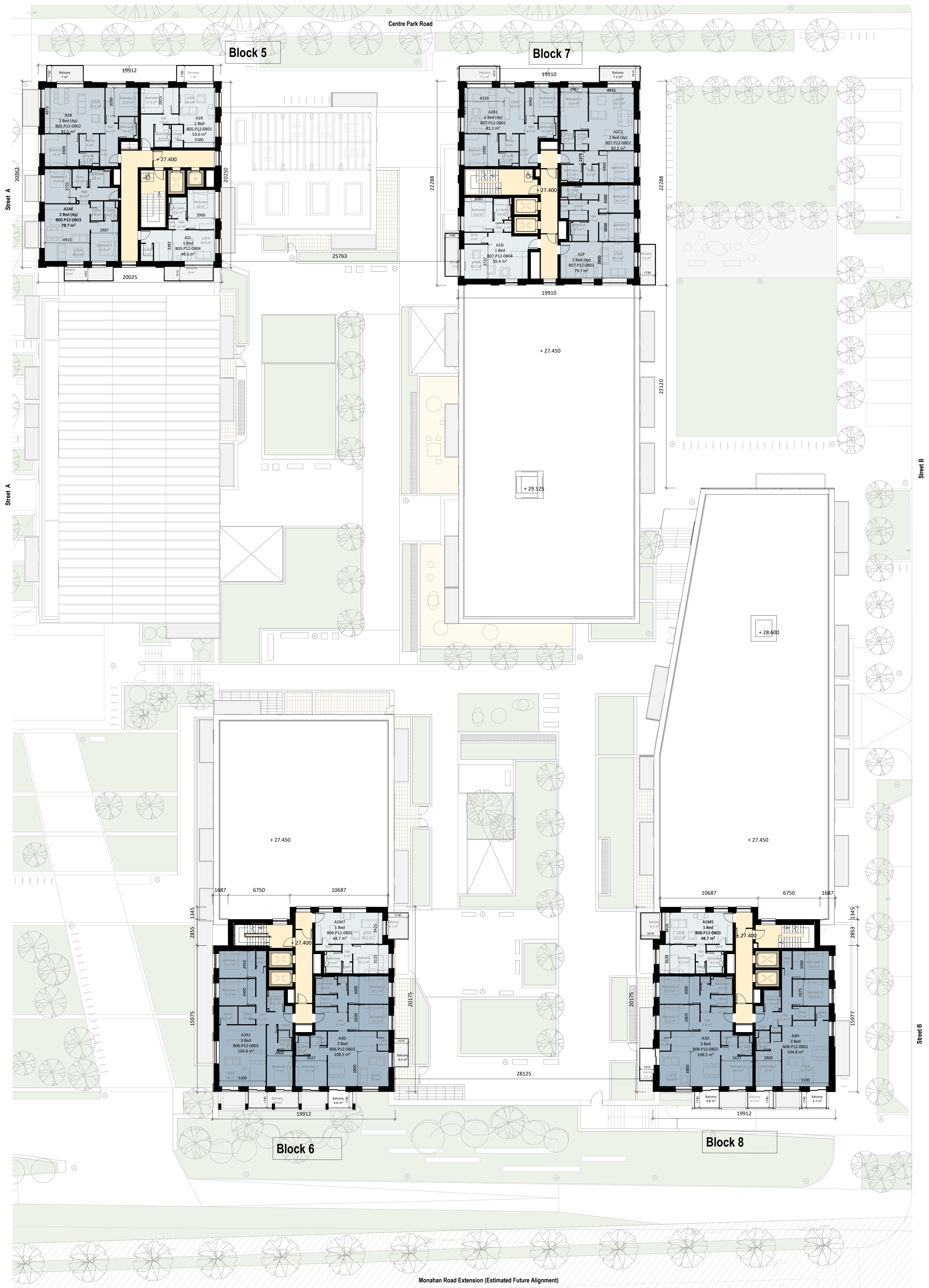
Podium 2 Level 08 Floor Plan
